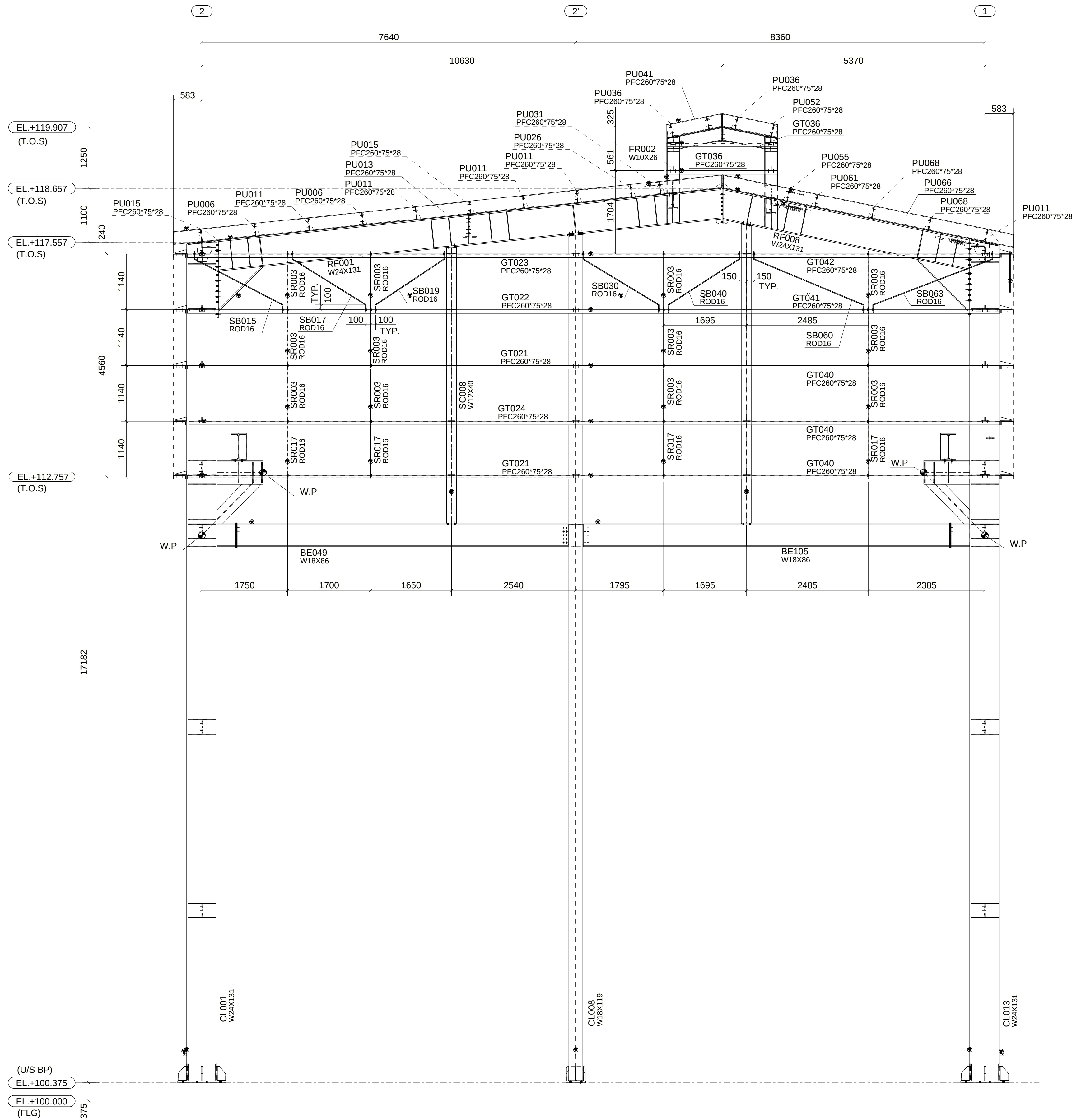
ELEVATION ALONG GRID-A (LOOKING TOWARDS NORTH) (GIRTS & PURLINS)
