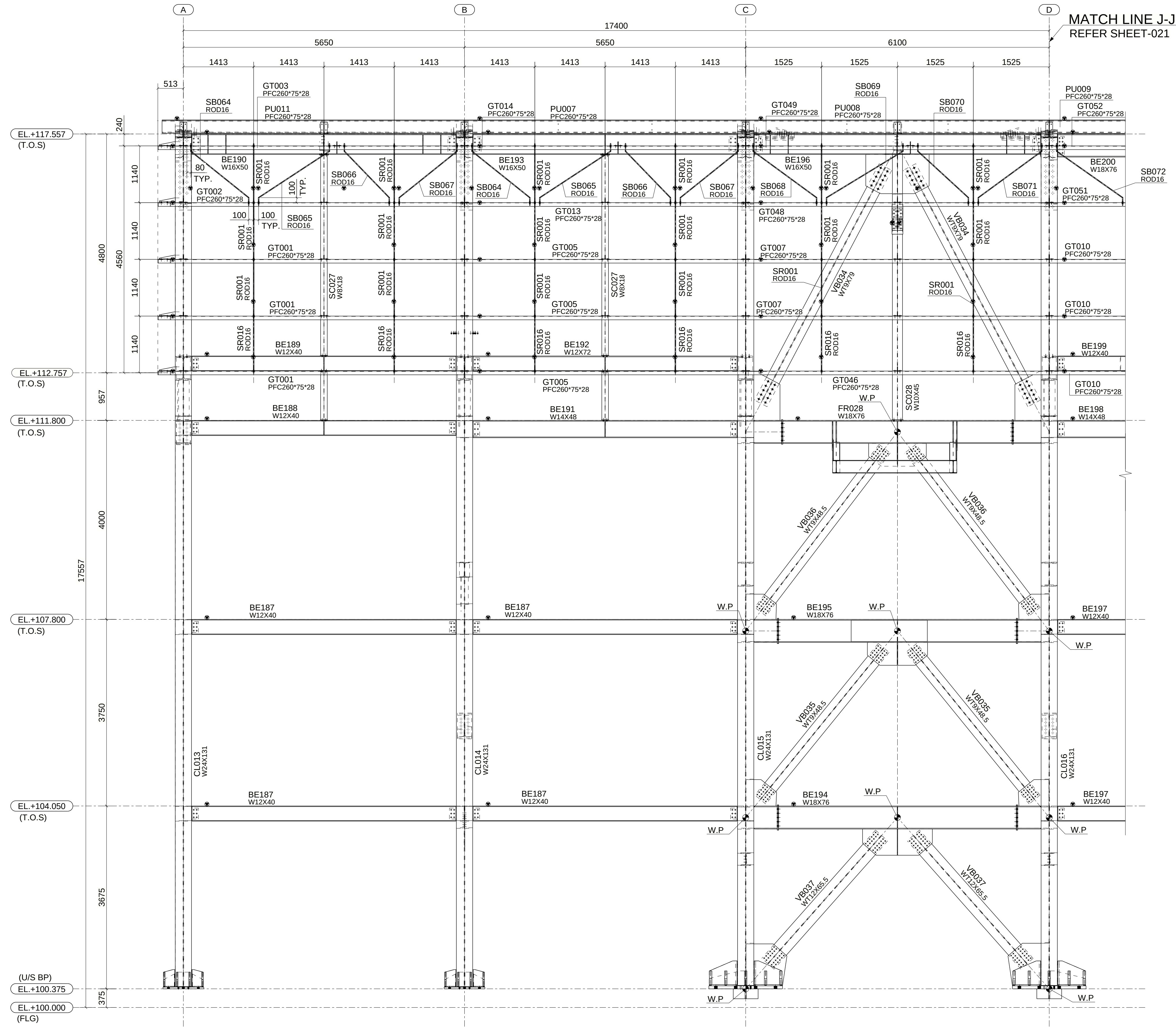
GIRT ELEVATION ALONG GRID-1 (LOOKING TOWARDS WEST) (GIRT ELEVATION)
