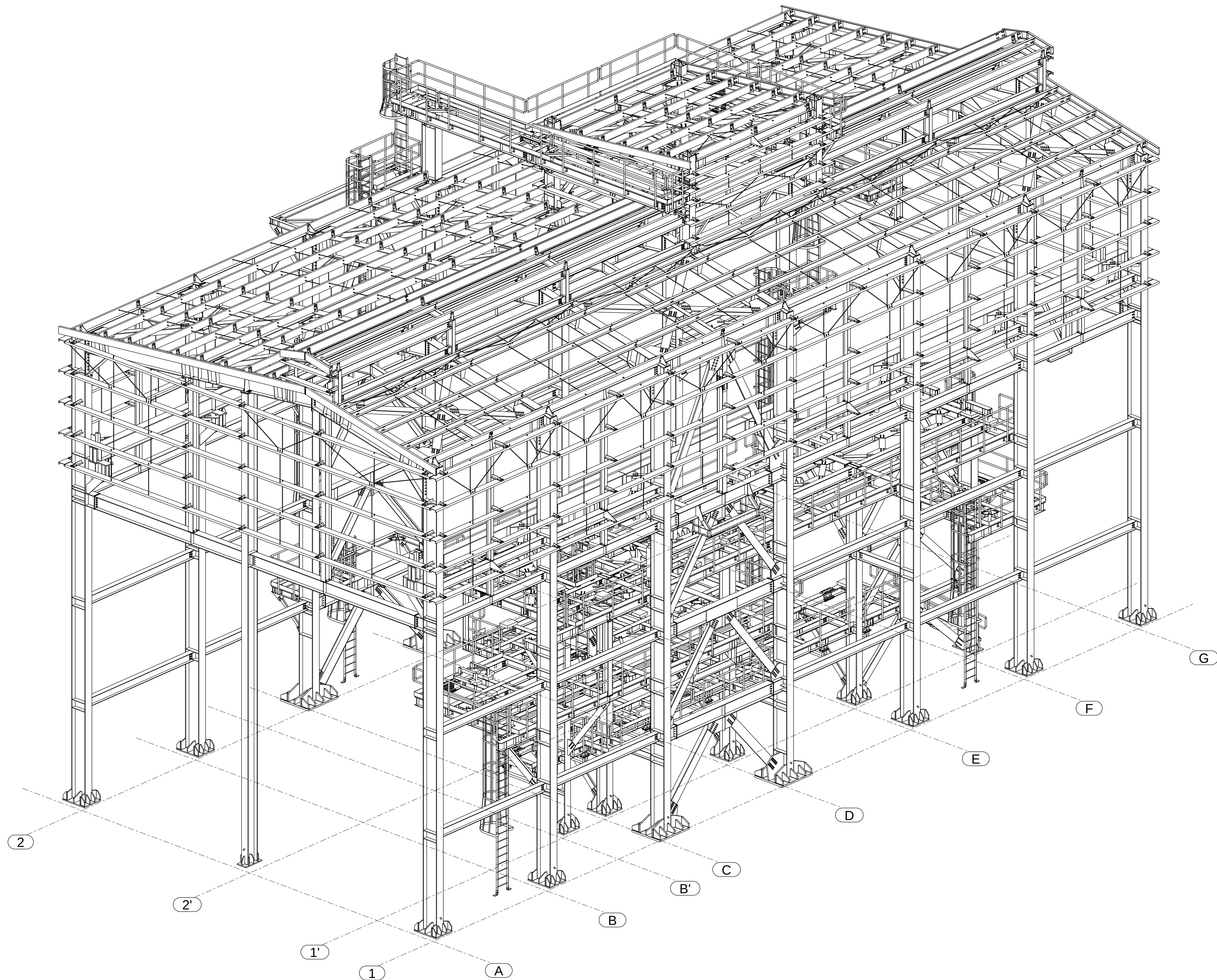
ISOMETRIC VIEW
